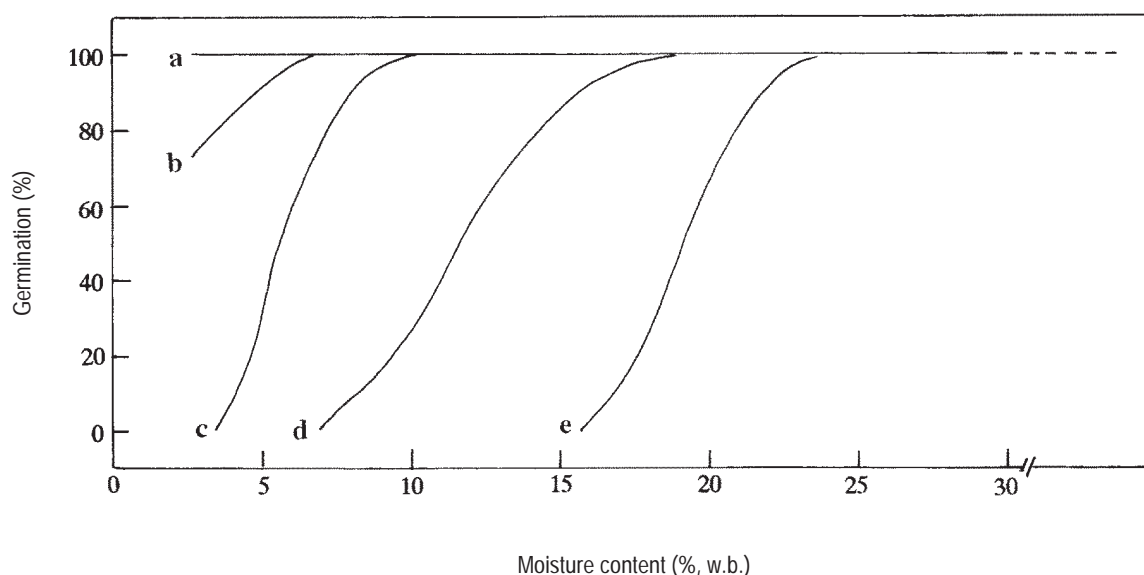
Fig. 1. The typical patterns of desiccation tolerance (normal germination, %, plotted against moisture content, % w.b.) are shown for species with orthodox (a), intermediate (c) and recalcitrant (e) seed storage behaviour. Two further patterns (b and d) are also shown which may be found in species with orthodox and intermediate seed storage behaviour, respectively, where the seed lot has been harvested prematurely or too late, or has been wrongly pretreated (see sections 4, 6.2.7 and 6.4). Seeds of some species with recalcitrant seed storage behaviour can be much more intolerant of desiccation than those shown by pattern e.
